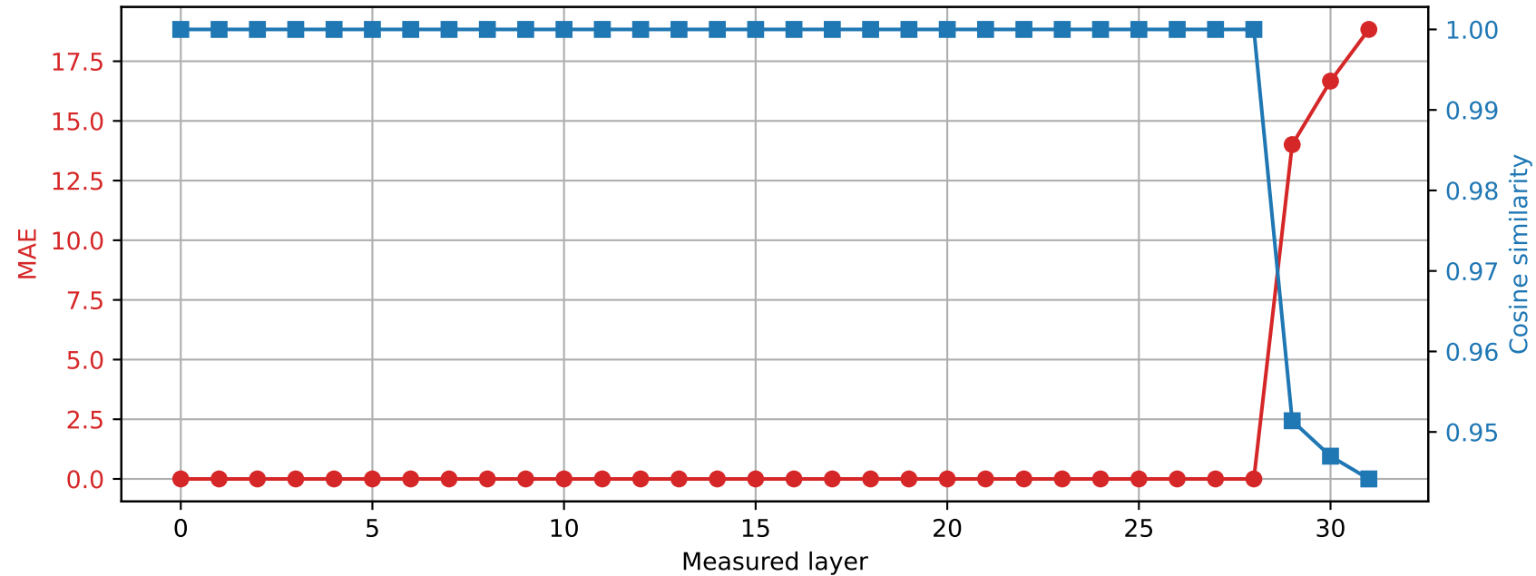
SmolLM2-360M | Prompt 3 Spared layer 28 | Hybrid vs quantized
