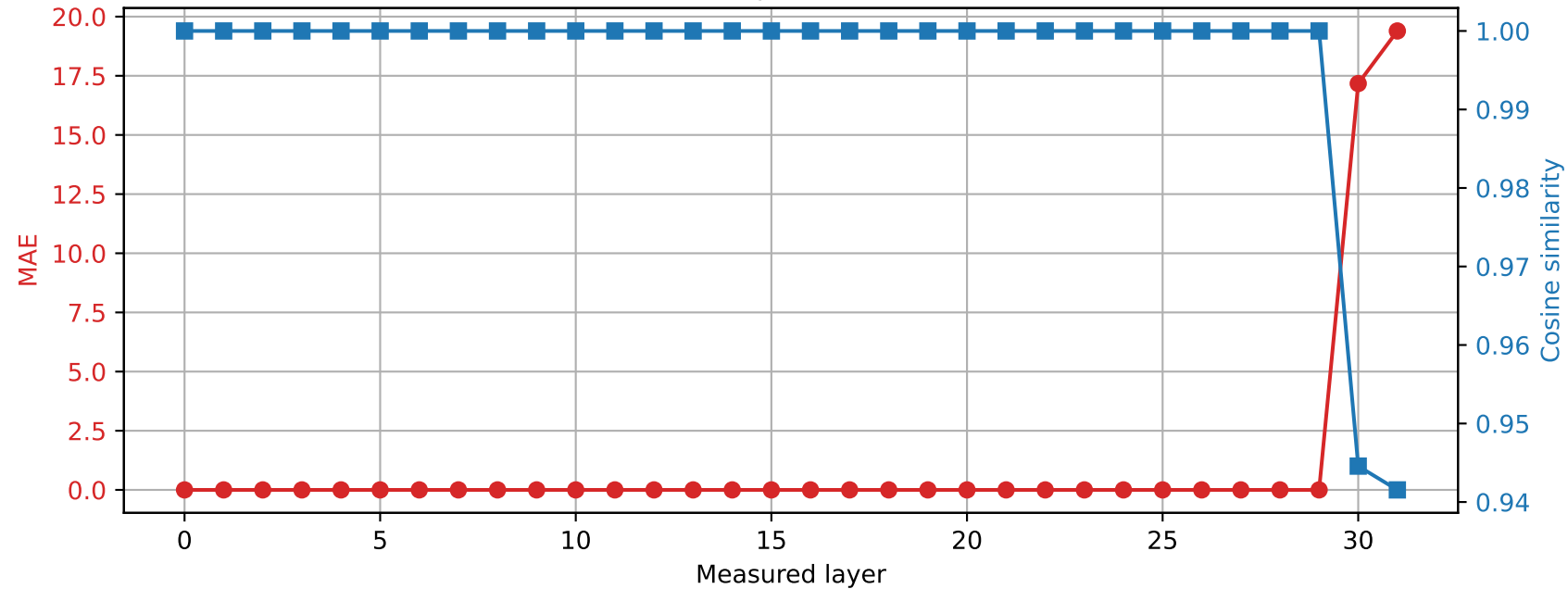
SmolLM2-360M | Prompt 3 Spared layer 29 | Hybrid vs quantized
