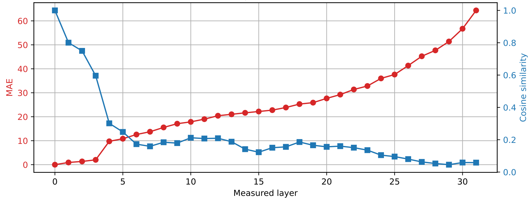
SmolLM2-360M | Prompt 4 Spared layer 3 | Hybrid vs unquantized
