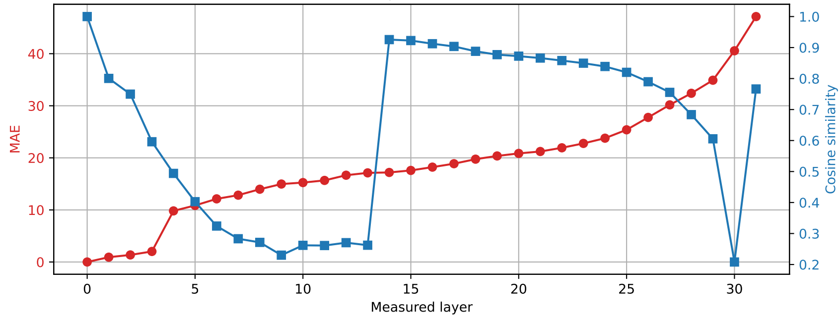
SmolLM2-360M | Prompt 4 Spared layer 9 | Hybrid vs unquantized
