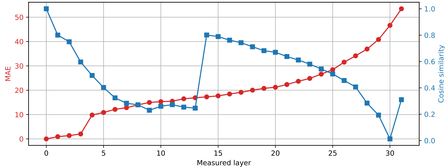
SmolLM2-360M | Prompt 4 Spared layer 10 | Hybrid vs unquantized
