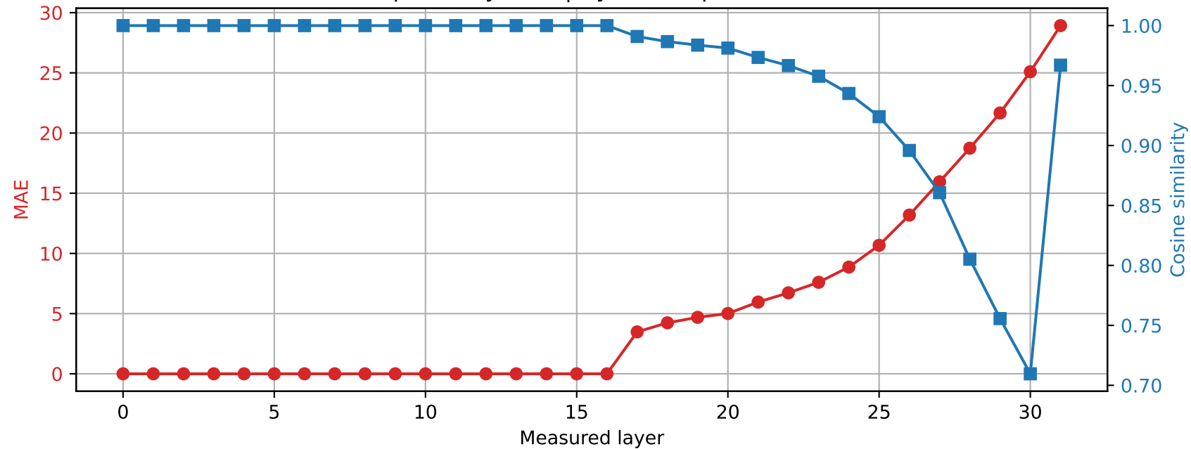
SmolLM2-360M | Prompt 4 Spared layer 16 | Hybrid vs quantized
