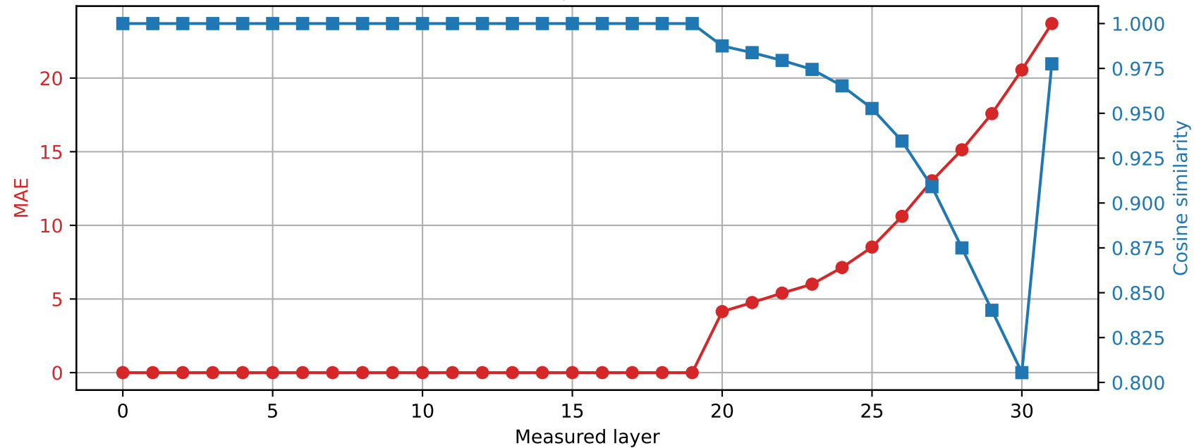
SmolLM2-360M | Prompt 4 Spared layer 19 | Hybrid vs quantized
