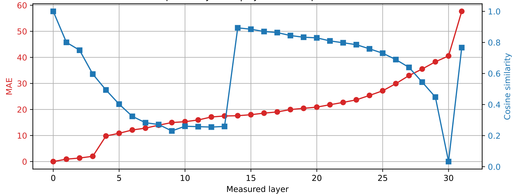
SmolLM2-360M | Prompt 4 Spared layer 29 | Hybrid vs unquantized
