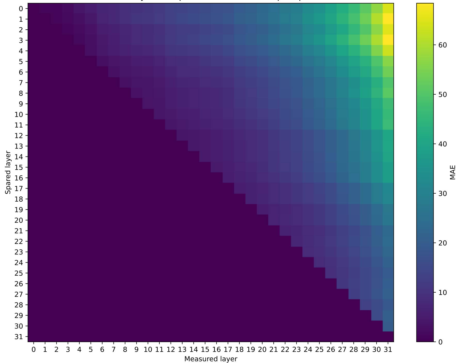
SmolLM2-360M Mean hybrid vs quantized MAE across 5 prompts
