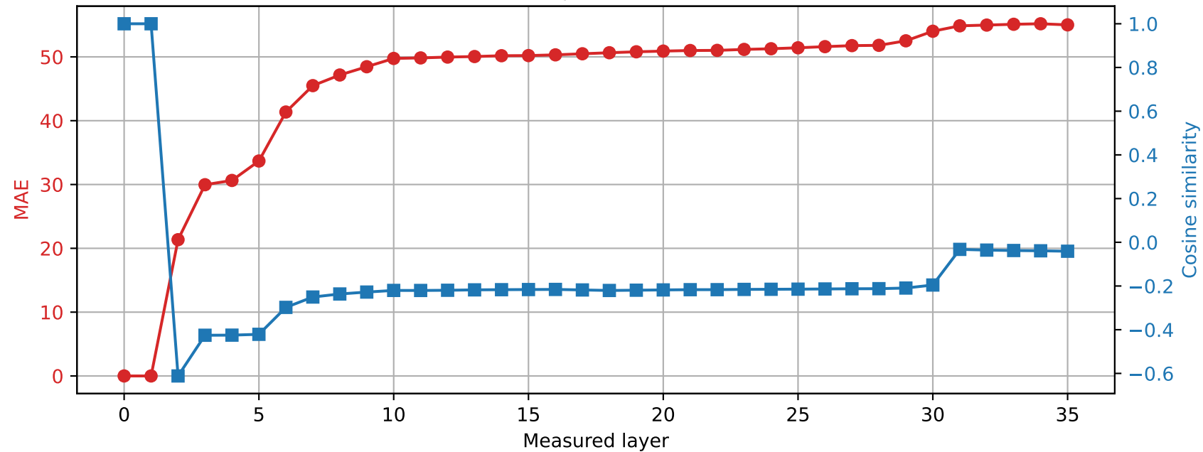
Qwen2.5-3B | Prompt 0 Spared layer 1 | Hybrid vs quantized
