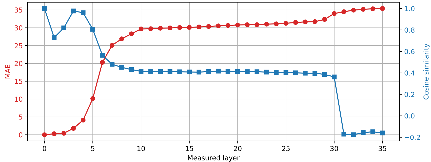
Qwen2.5-3B | Prompt 0 Spared layer 1 | Hybrid vs unquantized
