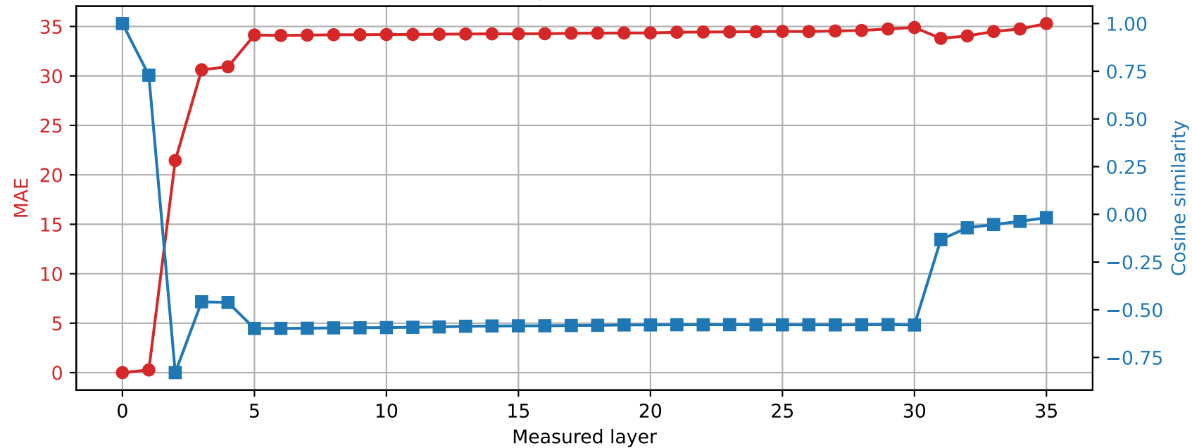
Qwen2.5-3B | Prompt 0 Spared layer 4 | Hybrid vs unquantized
