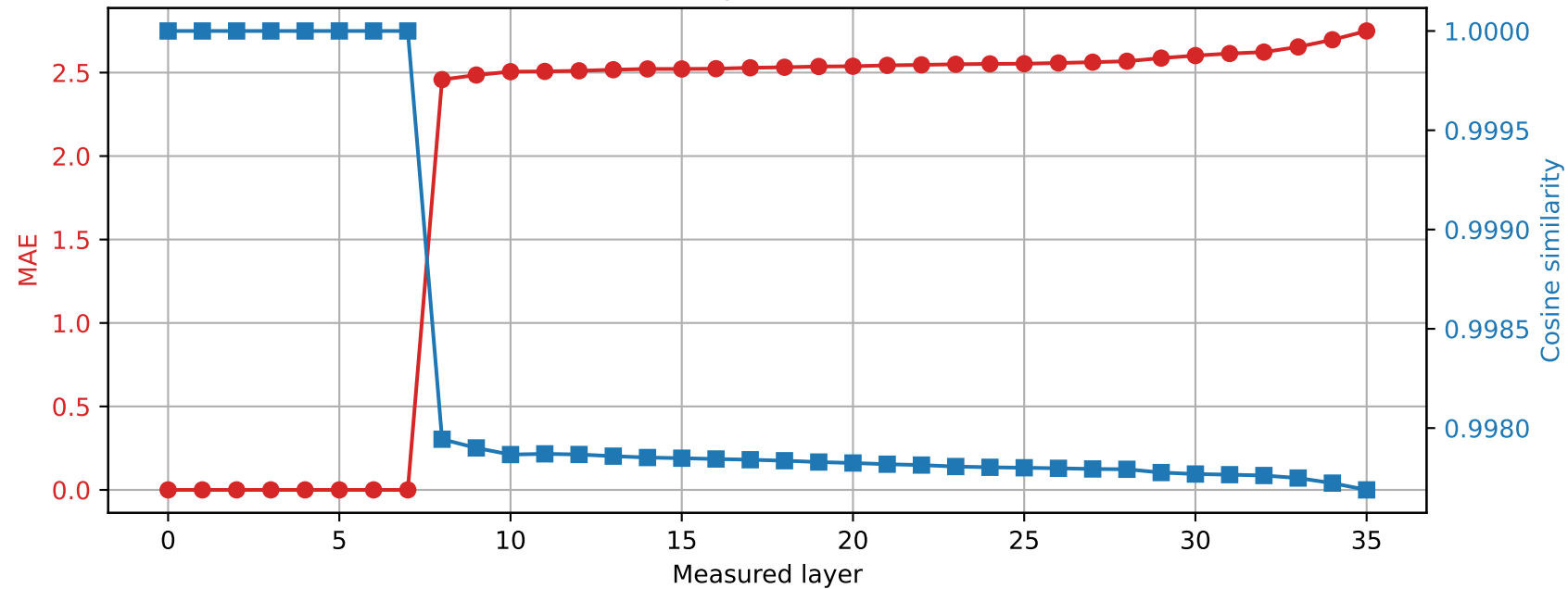
Qwen2.5-3B | Prompt 0 Spared layer 7 | Hybrid vs quantized
