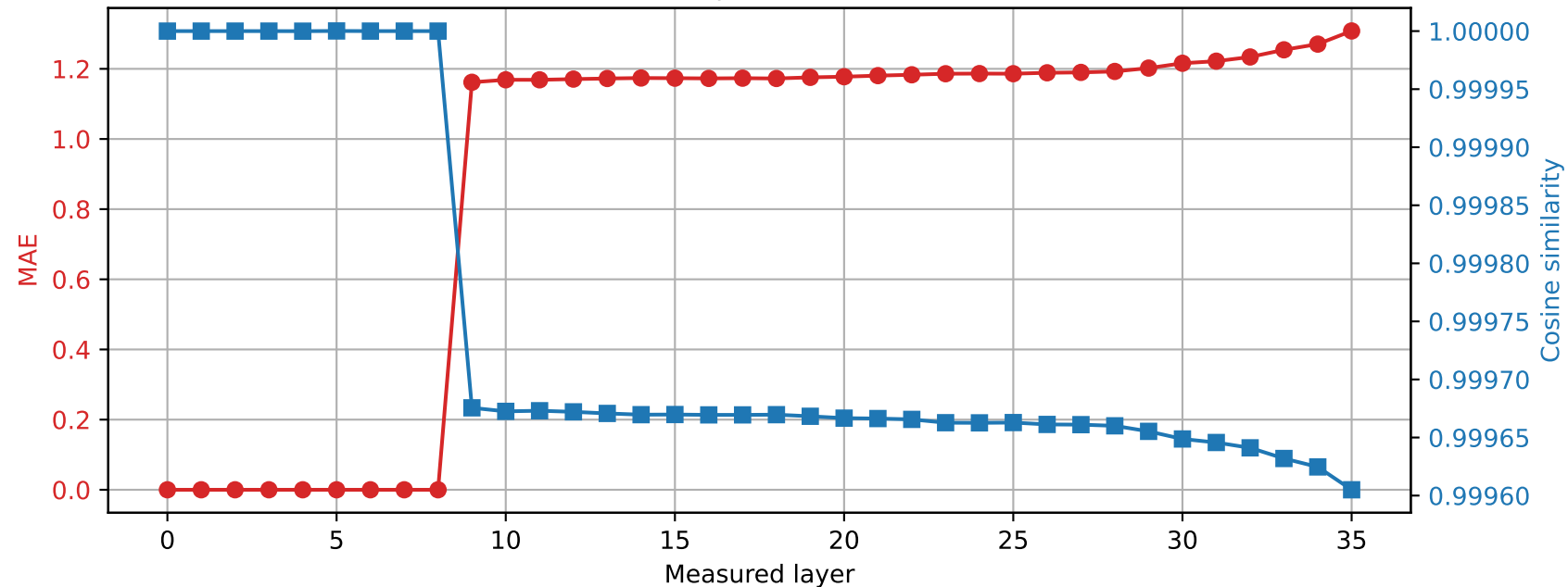
Qwen2.5-3B | Prompt 0 Spared layer 8 | Hybrid vs quantized
