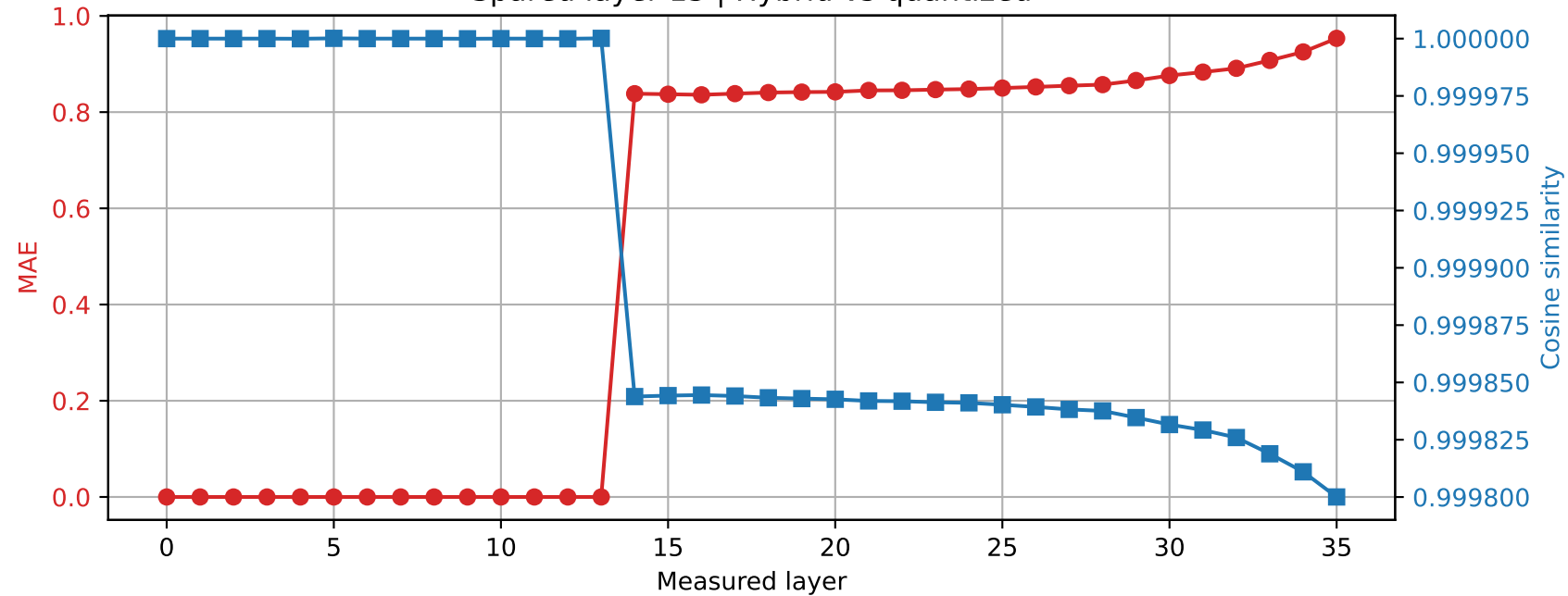
Qwen2.5-3B | Prompt 0 Spared layer 13 | Hybrid vs quantized
