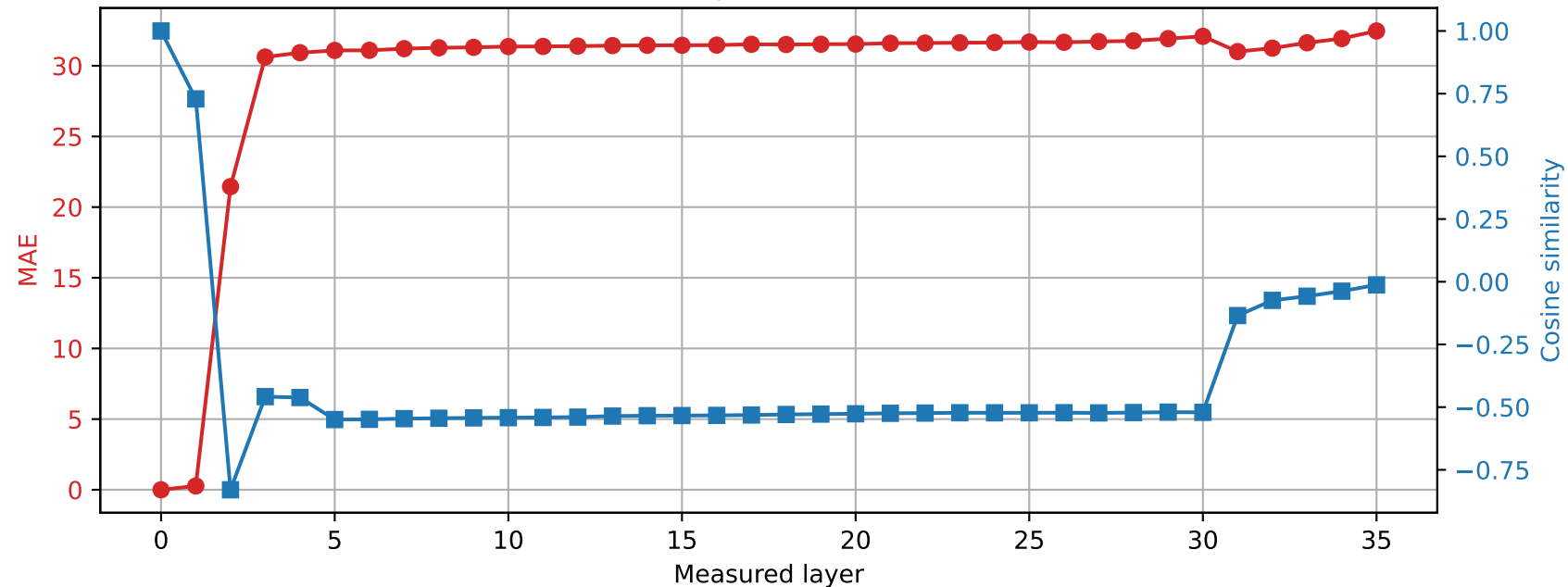
Qwen2.5-3B | Prompt 0 Spared layer 17 | Hybrid vs unquantized
