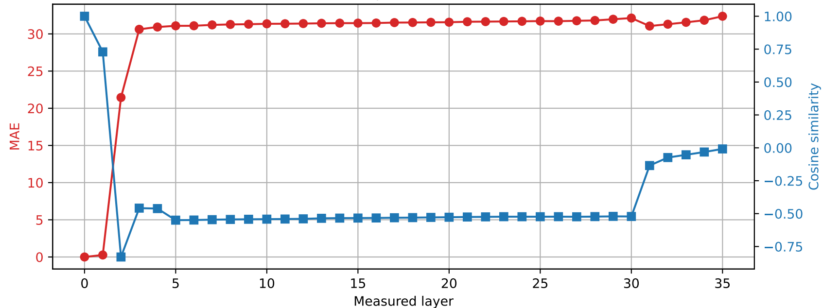
Qwen2.5-3B | Prompt 0 Spared layer 32 | Hybrid vs unquantized
