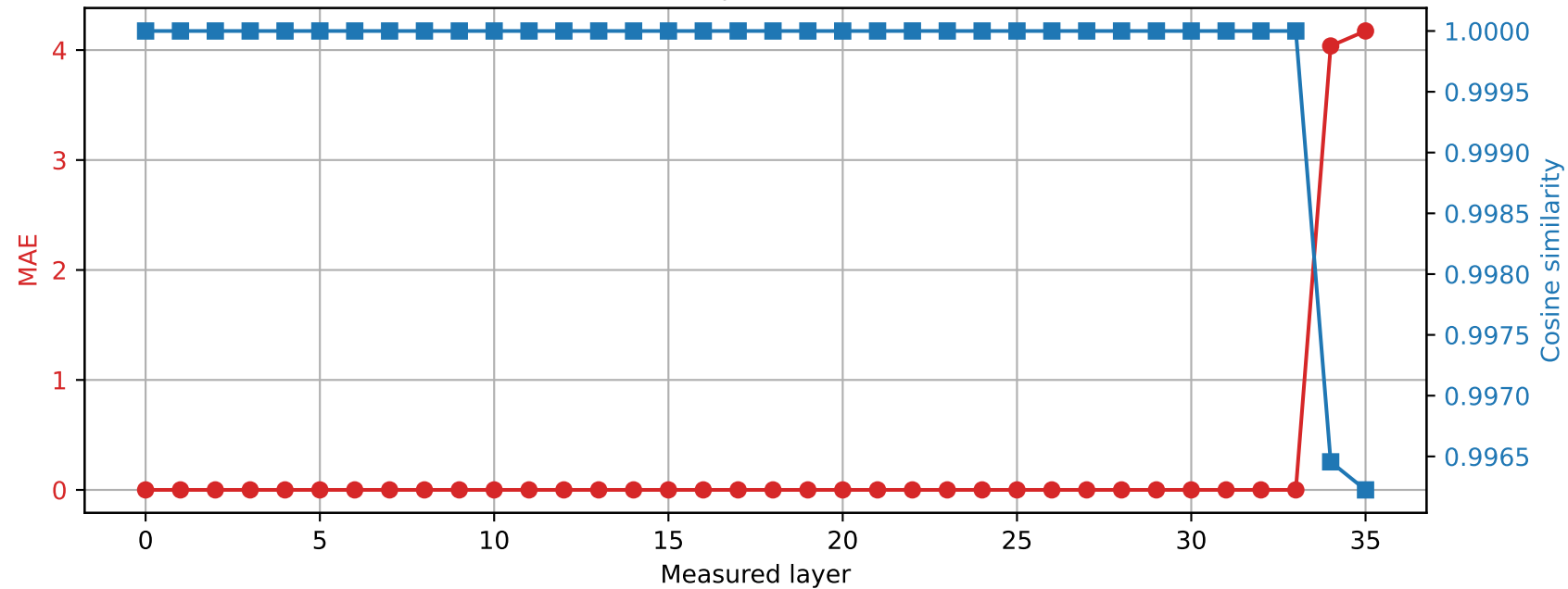
Qwen2.5-3B | Prompt 0 Spared layer 33 | Hybrid vs quantized
