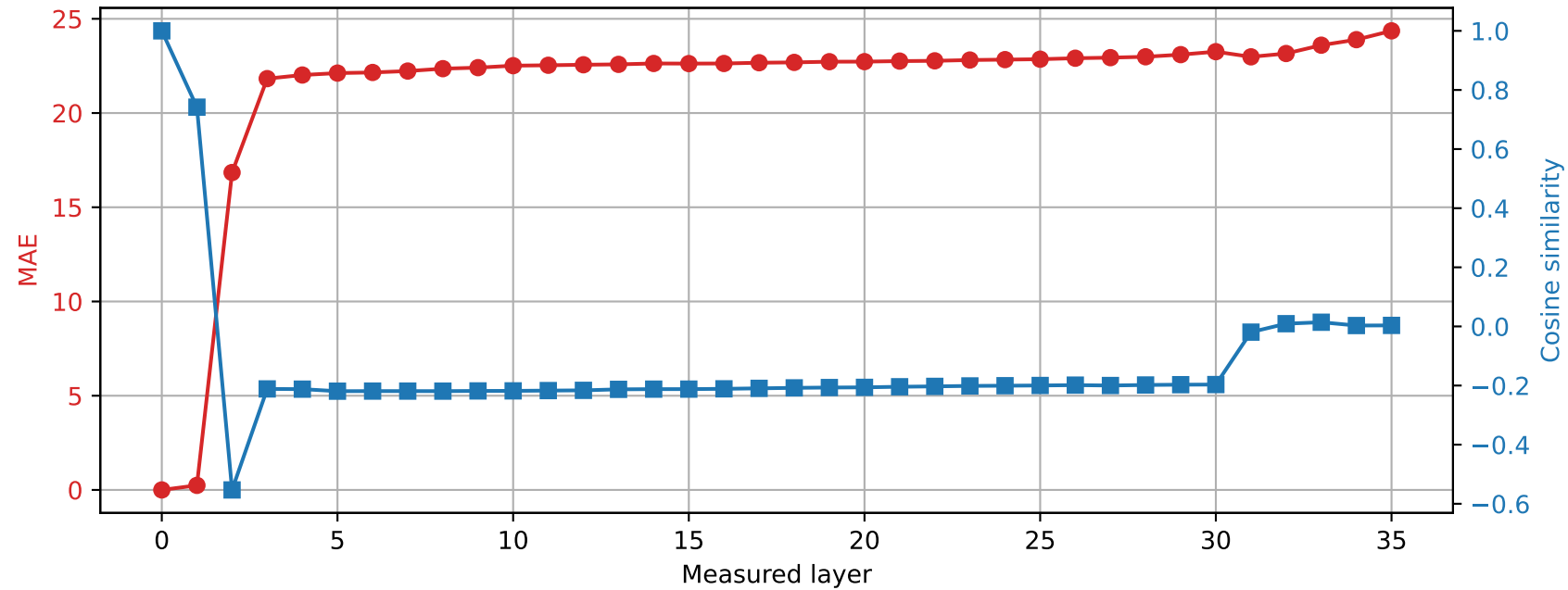
Qwen2.5-3B | Prompt 1 Unquantized vs quantized int4
