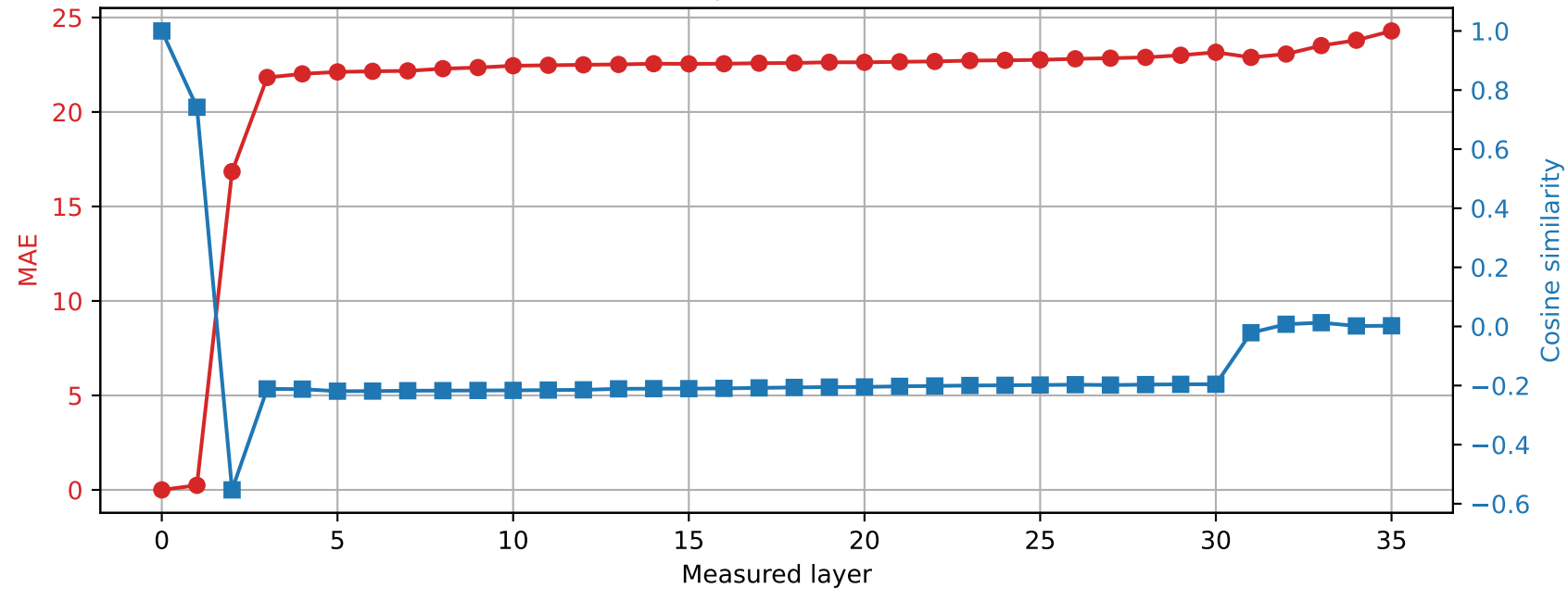
Qwen2.5-3B | Prompt 1 Spared layer 6 | Hybrid vs unquantized
