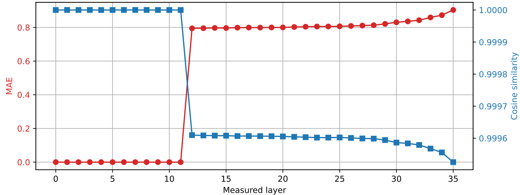
Qwen2.5-3B | Prompt 1 Spared layer 11 | Hybrid vs quantized
