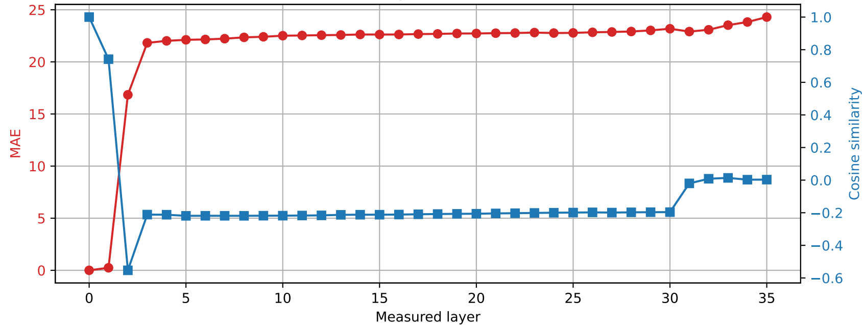
Qwen2.5-3B | Prompt 1 Spared layer 23 | Hybrid vs unquantized
