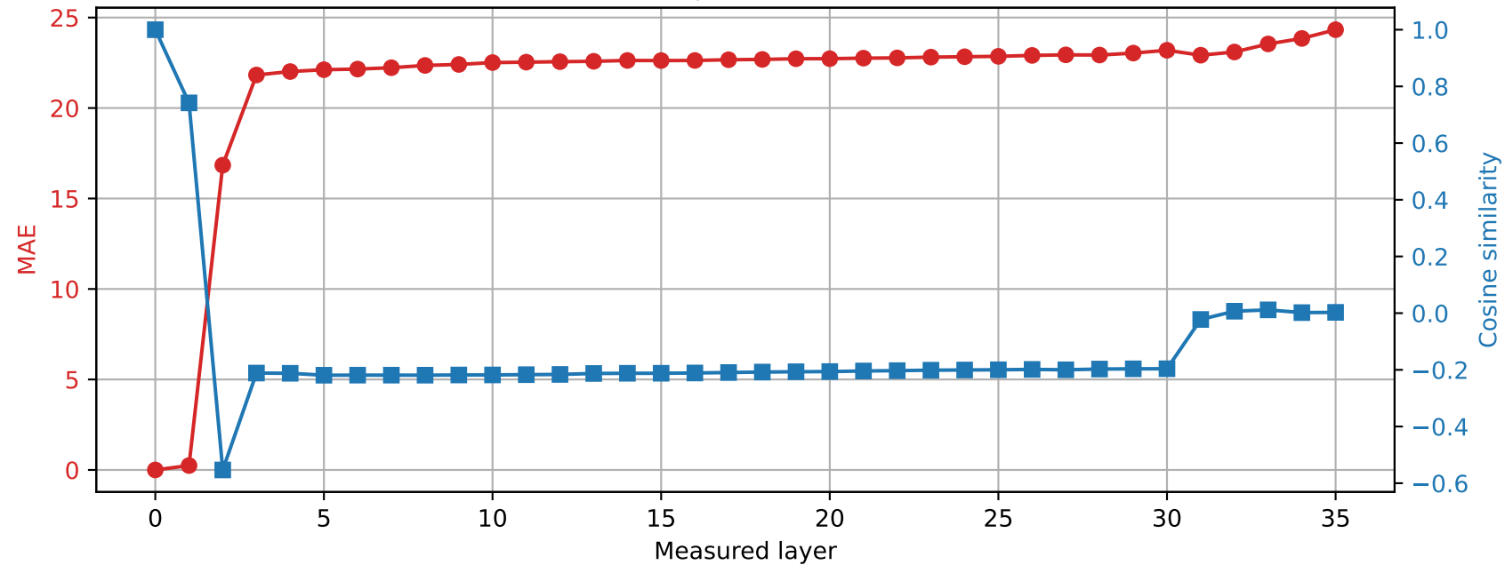
Qwen2.5-3B | Prompt 1 Spared layer 27 | Hybrid vs unquantized
