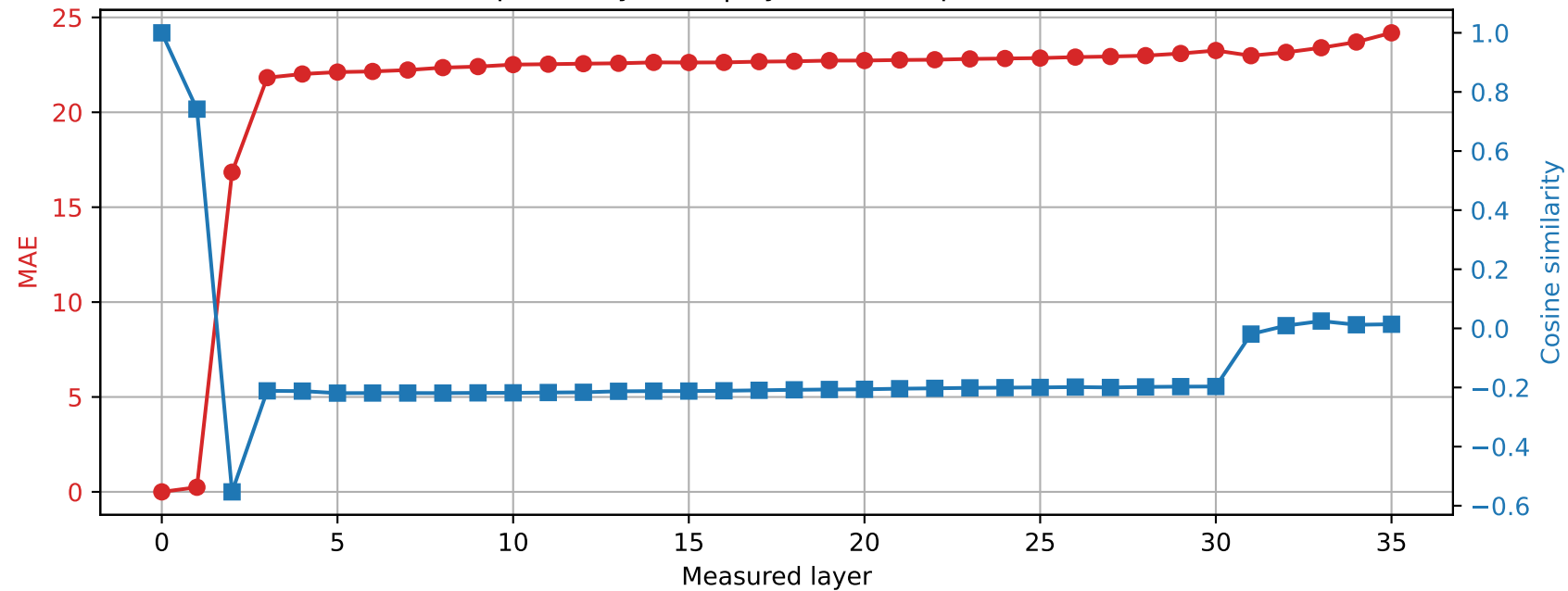
Qwen2.5-3B | Prompt 1 Spared layer 32 | Hybrid vs unquantized
