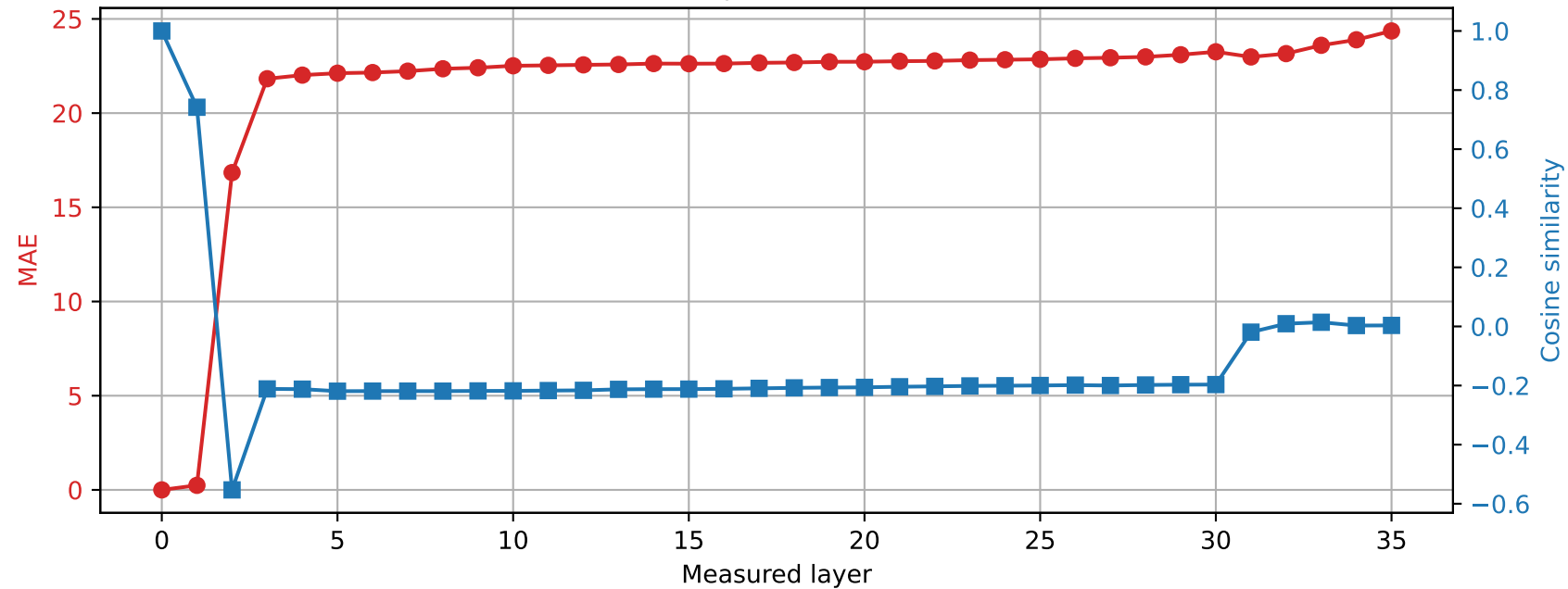
Qwen2.5-3B | Prompt 1 Spared layer 35 | Hybrid vs unquantized
