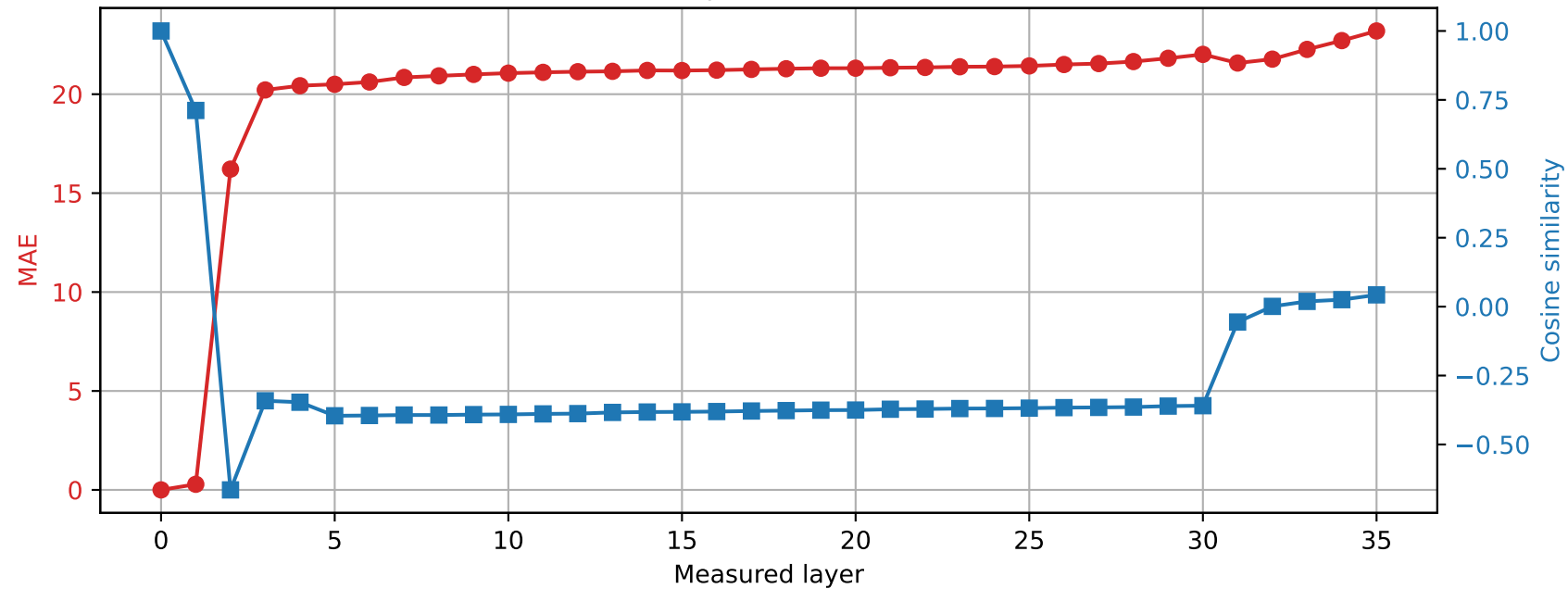
Qwen2.5-3B | Prompt 2 Spared layer 7 | Hybrid vs unquantized
