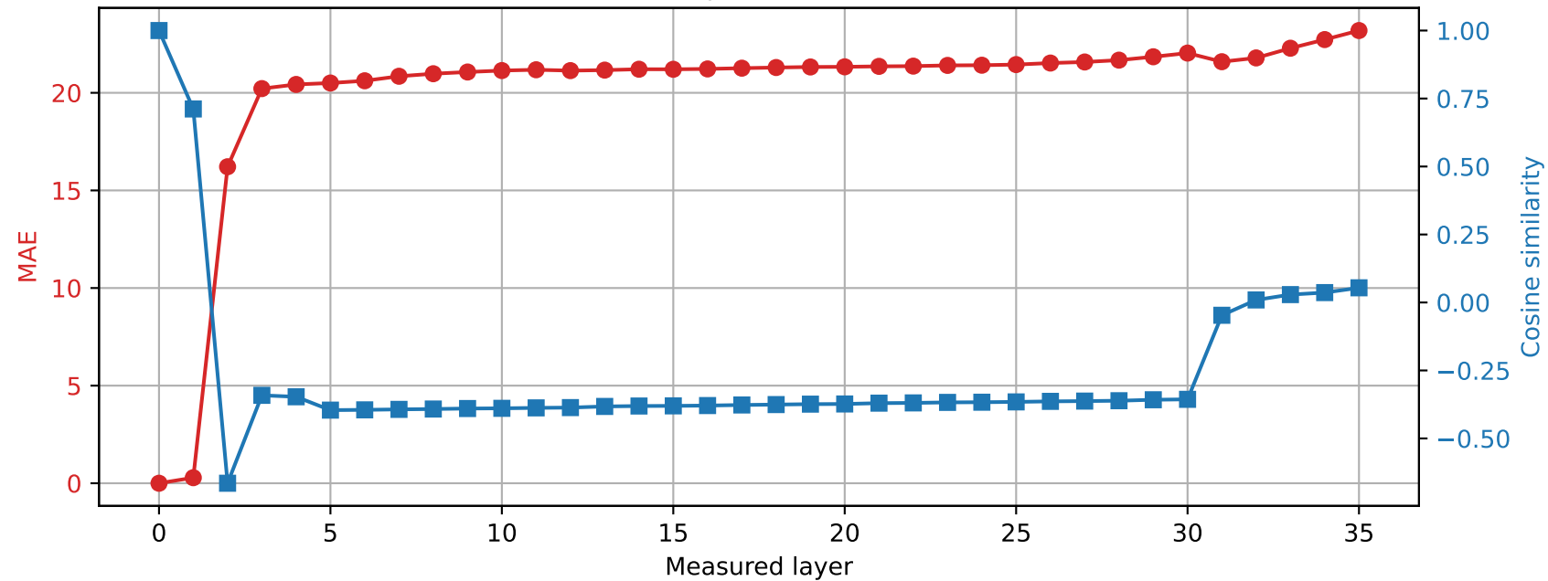
Qwen2.5-3B | Prompt 2 Spared layer 11 | Hybrid vs unquantized
