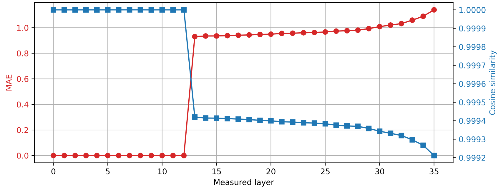
Qwen2.5-3B | Prompt 2 Spared layer 12 | Hybrid vs quantized
