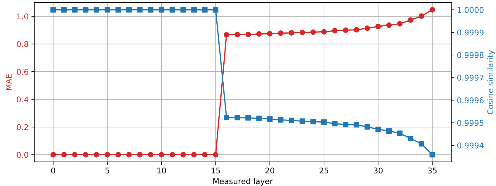
Qwen2.5-3B | Prompt 2 Spared layer 15 | Hybrid vs quantized
