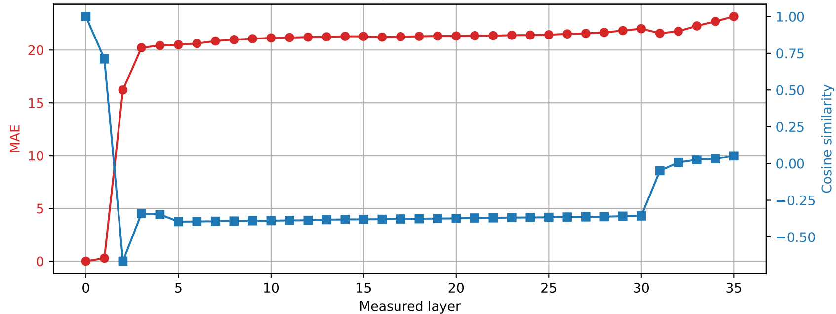
Qwen2.5-3B | Prompt 2 Spared layer 15 | Hybrid vs unquantized
