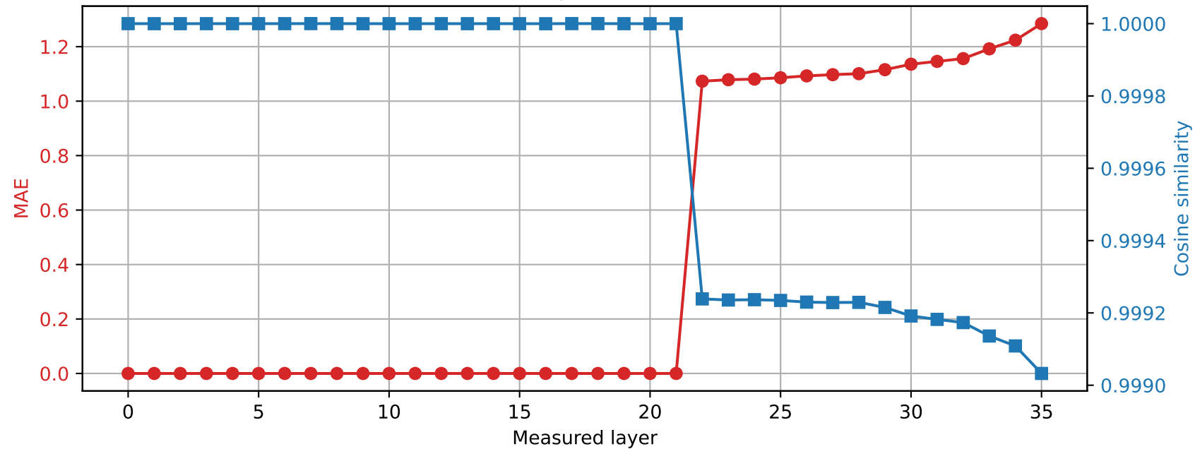
Qwen2.5-3B | Prompt 2 Spared layer 21 | Hybrid vs quantized
