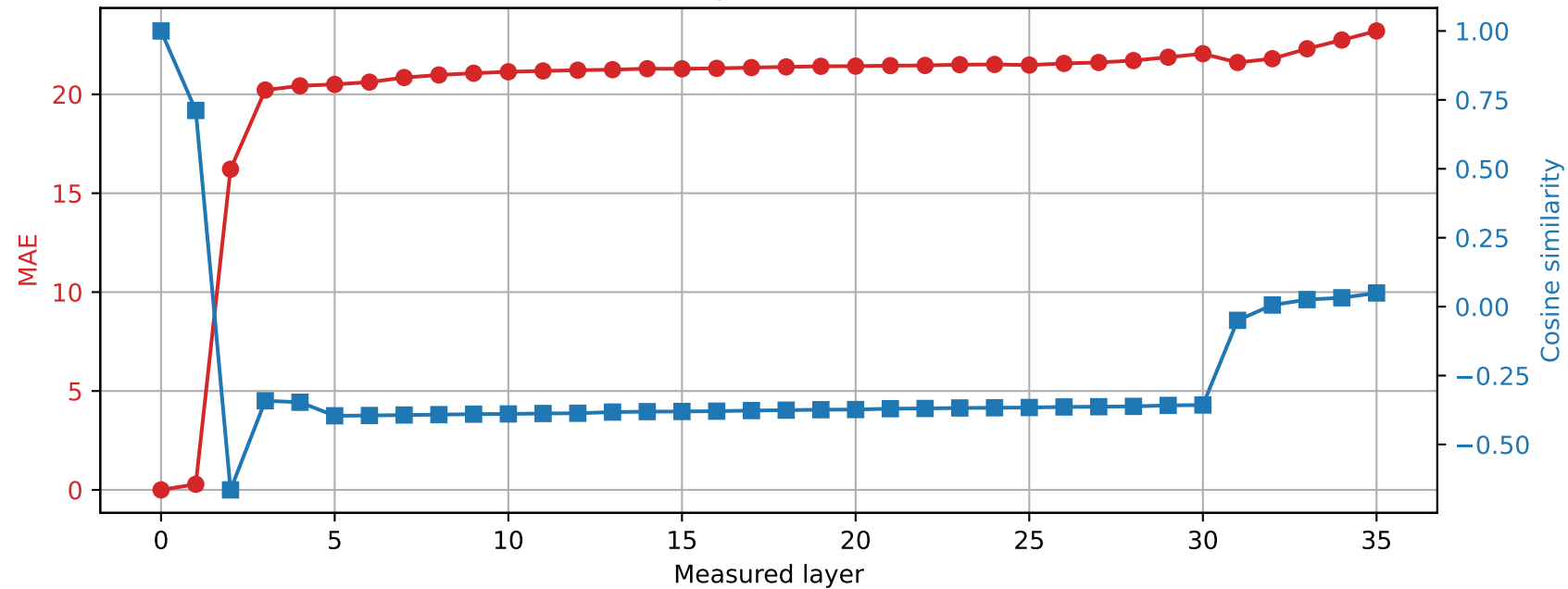
Qwen2.5-3B | Prompt 2 Spared layer 24 | Hybrid vs unquantized
