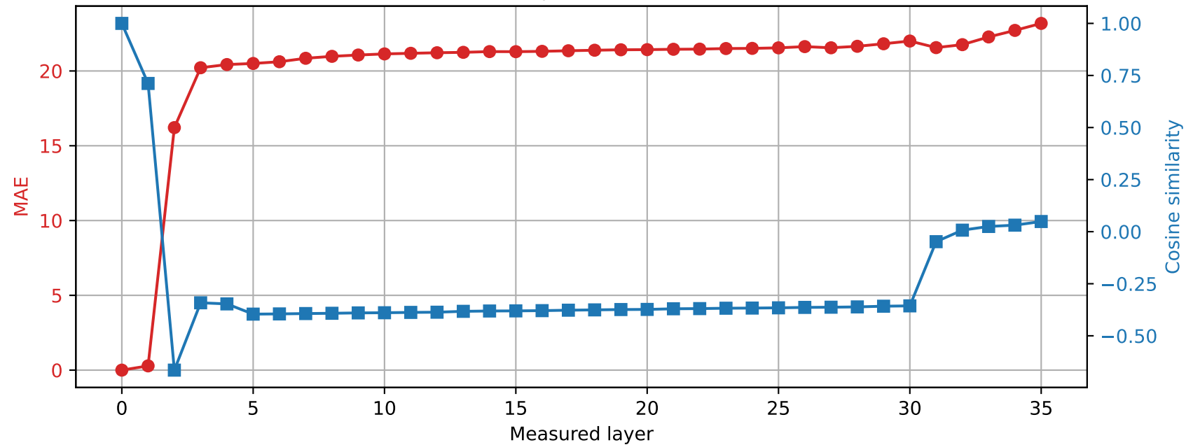
Qwen2.5-3B | Prompt 2 Spared layer 26 | Hybrid vs unquantized
