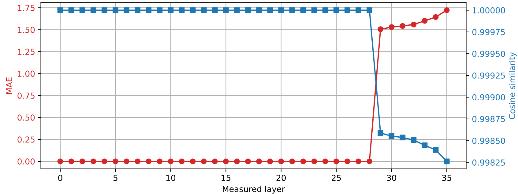
Qwen2.5-3B | Prompt 2 Spared layer 28 | Hybrid vs quantized
