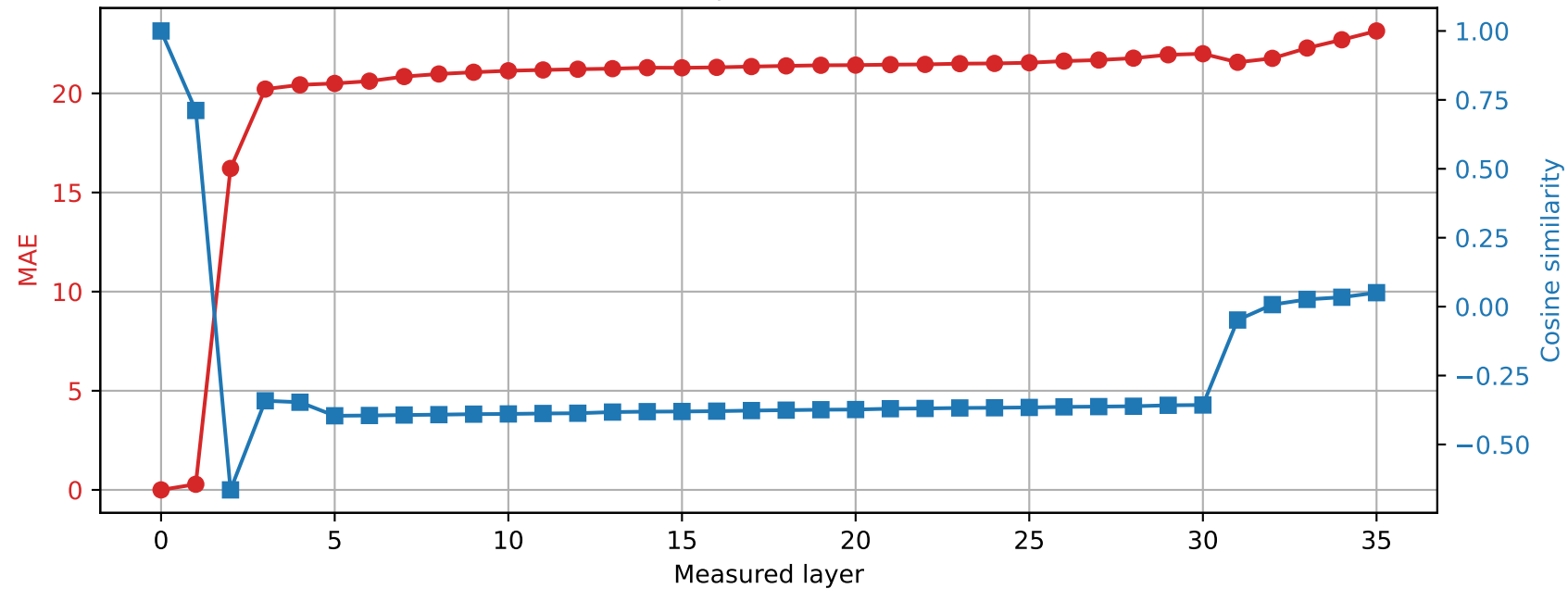
Qwen2.5-3B | Prompt 2 Spared layer 29 | Hybrid vs unquantized
