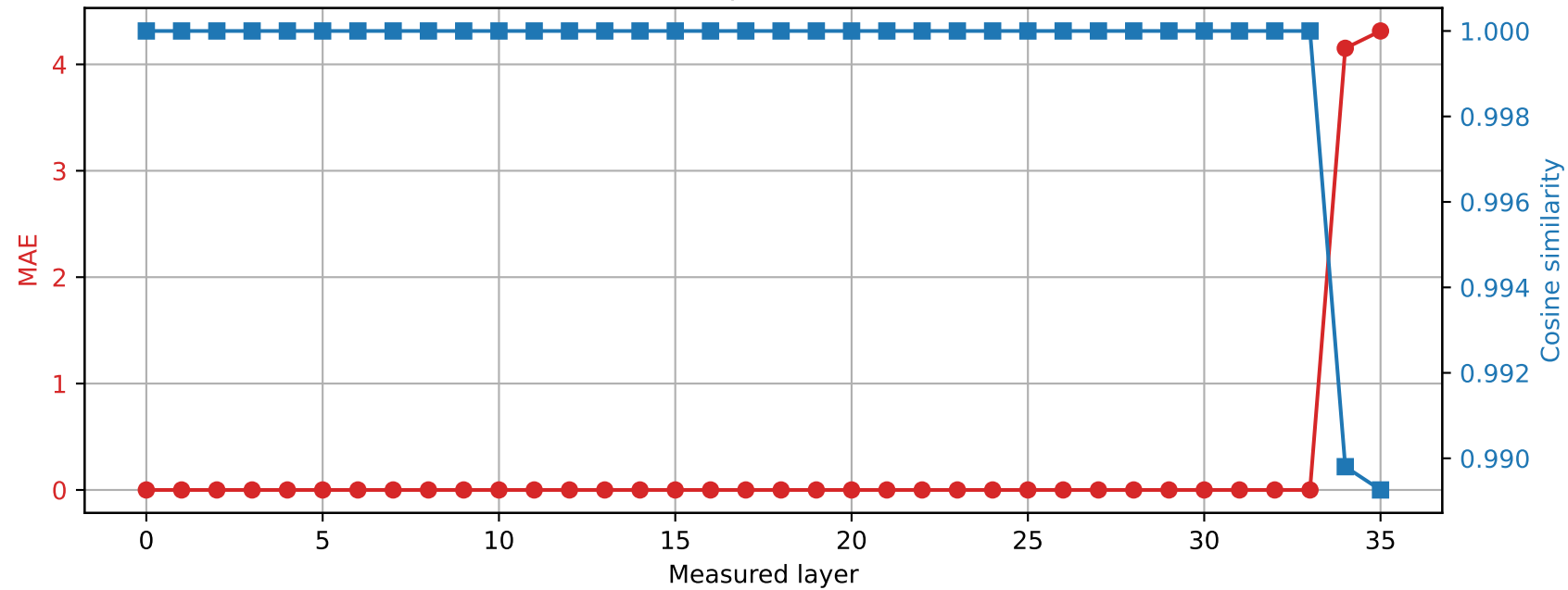
Qwen2.5-3B | Prompt 2 Spared layer 33 | Hybrid vs quantized
