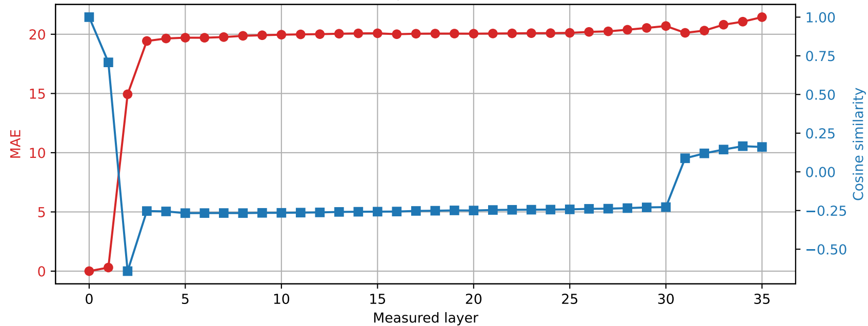
Qwen2.5-3B | Prompt 3 Spared layer 15 | Hybrid vs unquantized
