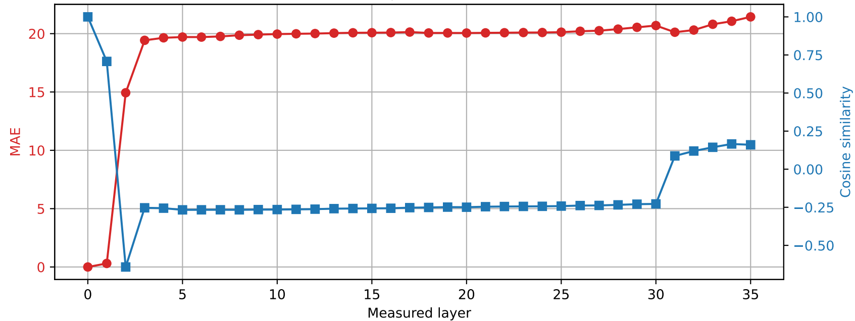
Qwen2.5-3B | Prompt 3 Spared layer 17 | Hybrid vs unquantized
