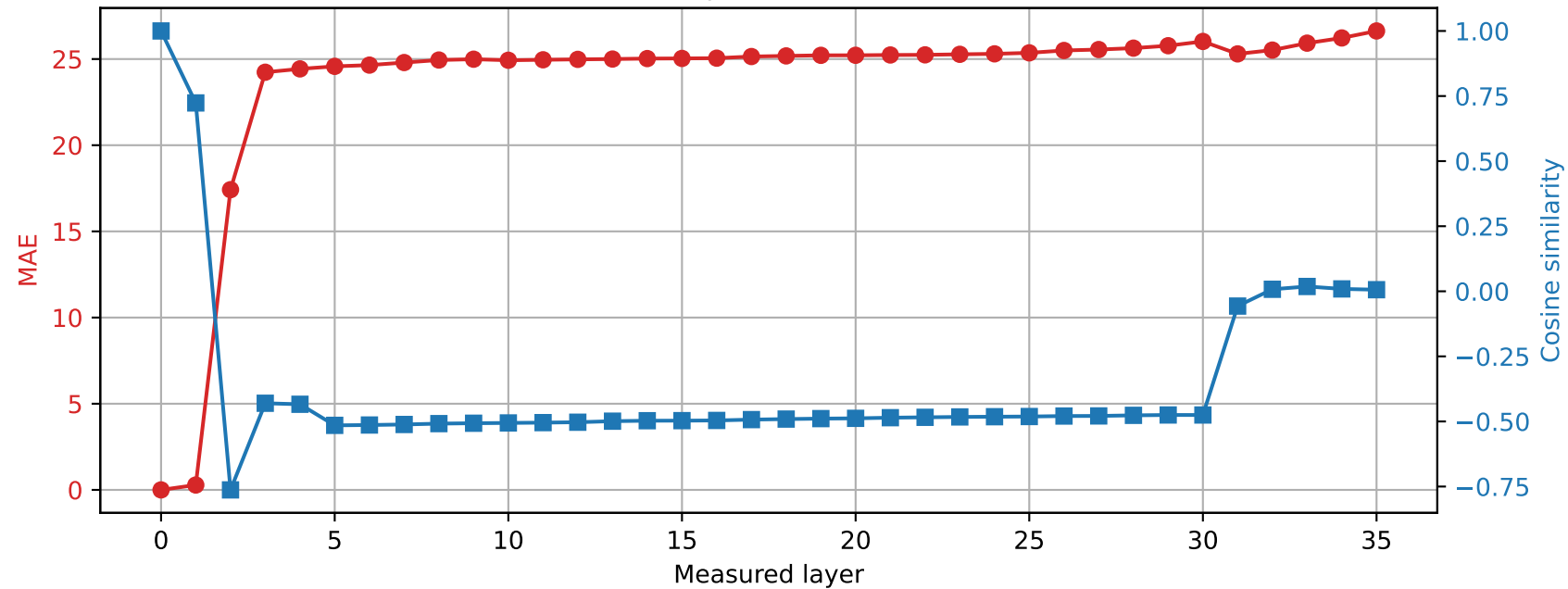
Qwen2.5-3B | Prompt 4 Spared layer 9 | Hybrid vs unquantized
