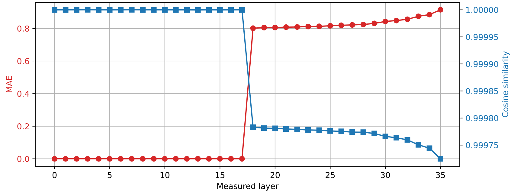
Qwen2.5-3B | Prompt 4 Spared layer 17 | Hybrid vs quantized
