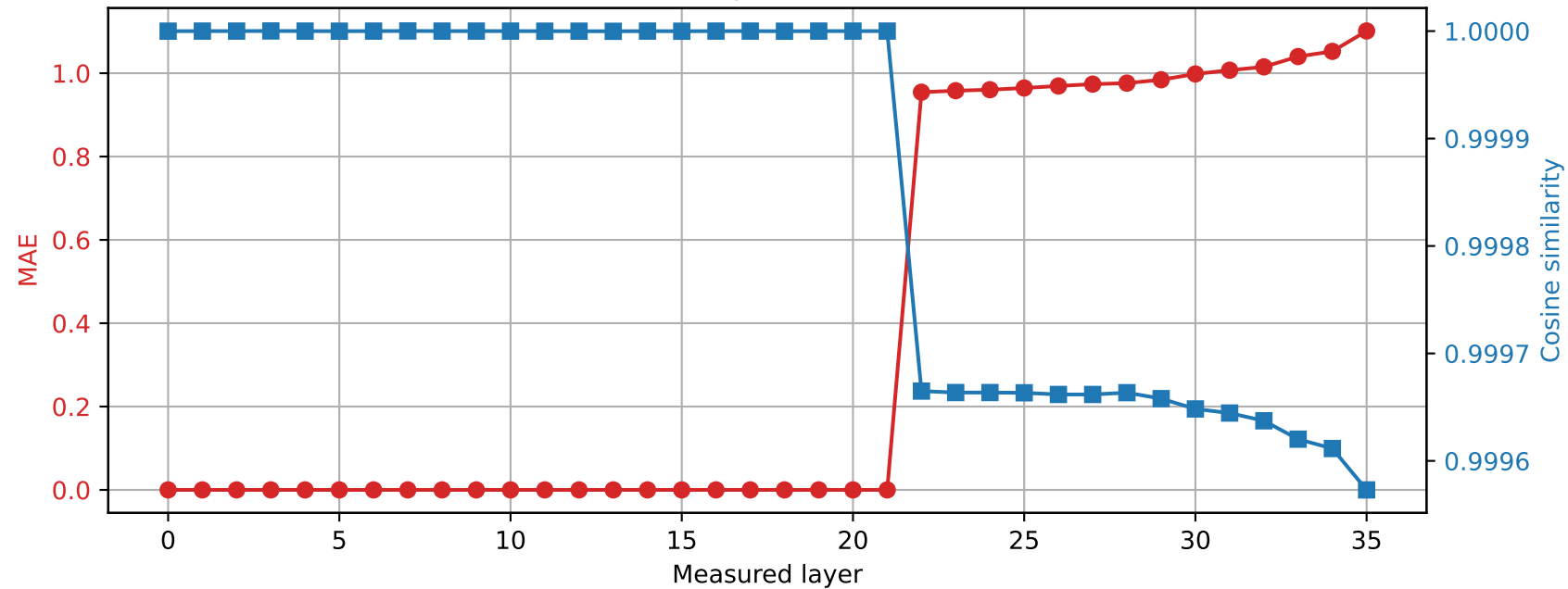
Qwen2.5-3B | Prompt 4 Spared layer 21 | Hybrid vs quantized
