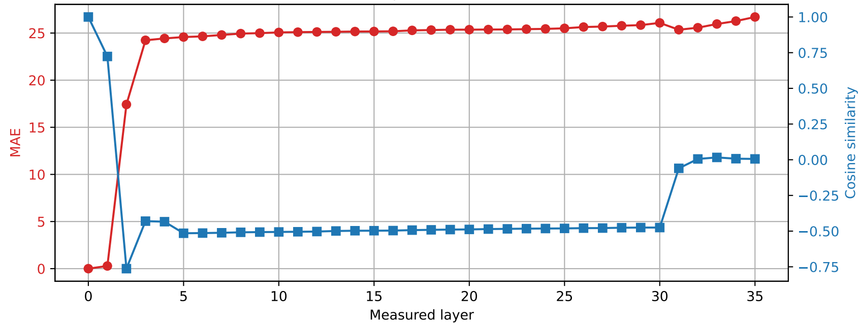
Qwen2.5-3B | Prompt 4 Spared layer 28 | Hybrid vs unquantized
