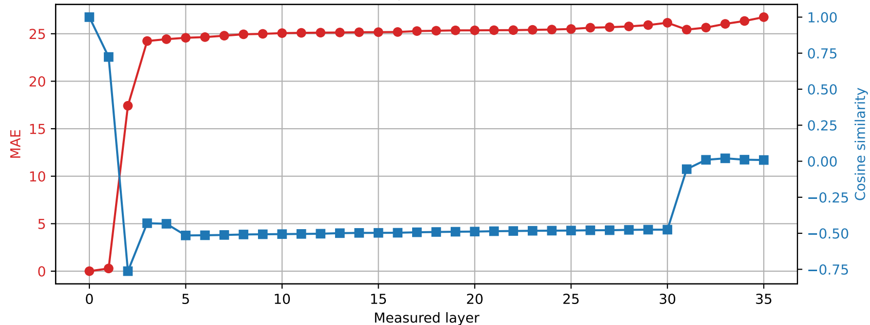
Qwen2.5-3B | Prompt 4 Spared layer 35 | Hybrid vs unquantized
