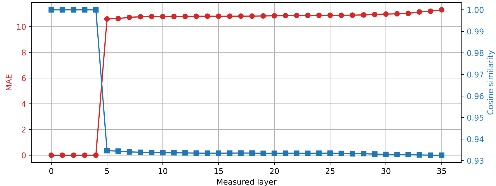
Qwen2.5-3B | Prompt 0 Spared layer 4 | Hybrid vs quantized
