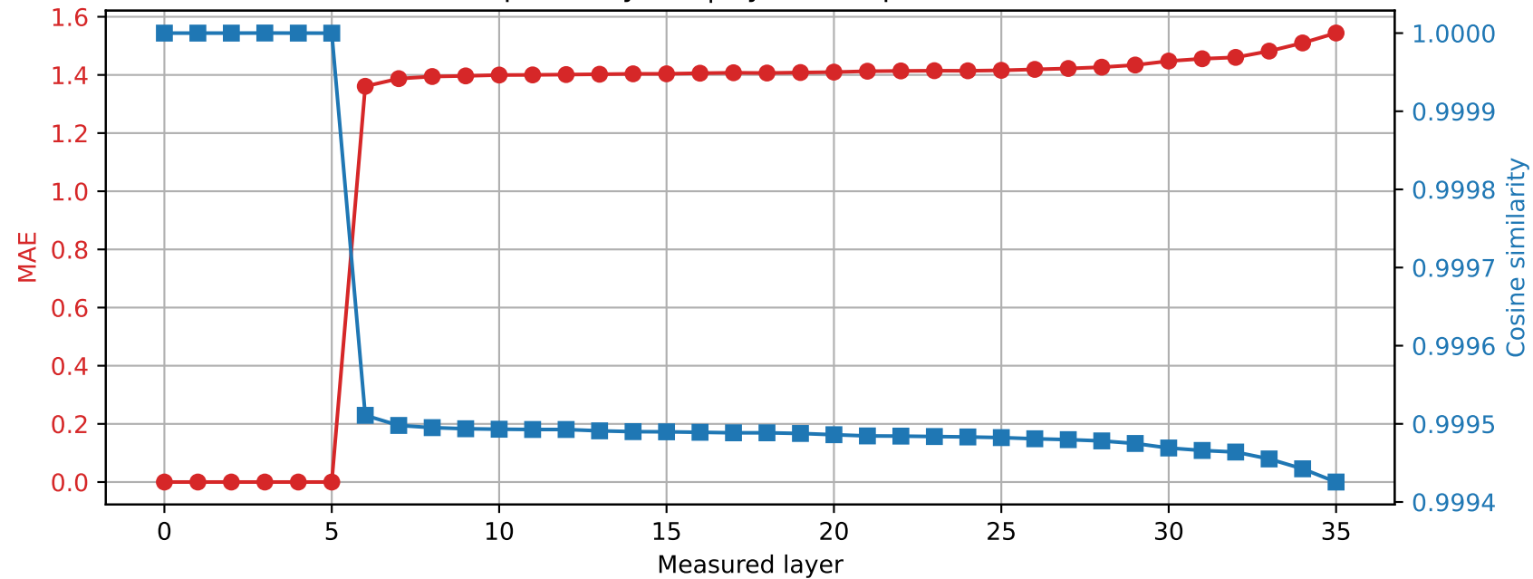
Qwen2.5-3B | Prompt 0 Spared layer 5 | Hybrid vs quantized
