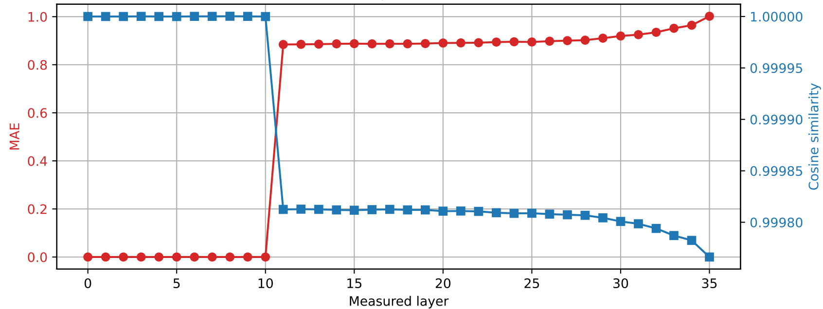
Qwen2.5-3B | Prompt 0 Spared layer 10 | Hybrid vs quantized
