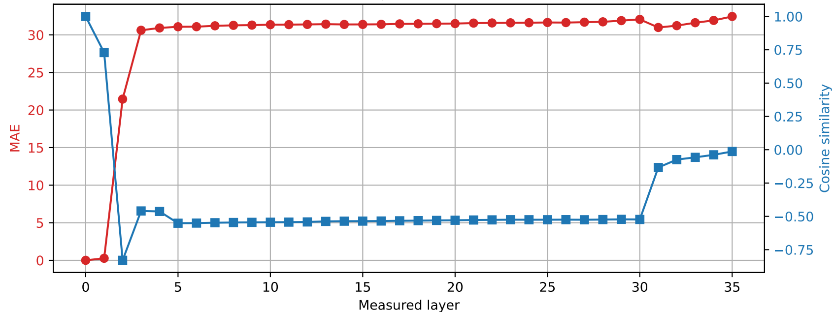
Qwen2.5-3B | Prompt 0 Spared layer 13 | Hybrid vs unquantized
