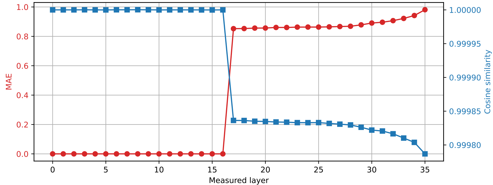
Qwen2.5-3B | Prompt 0 Spared layer 16 | Hybrid vs quantized
