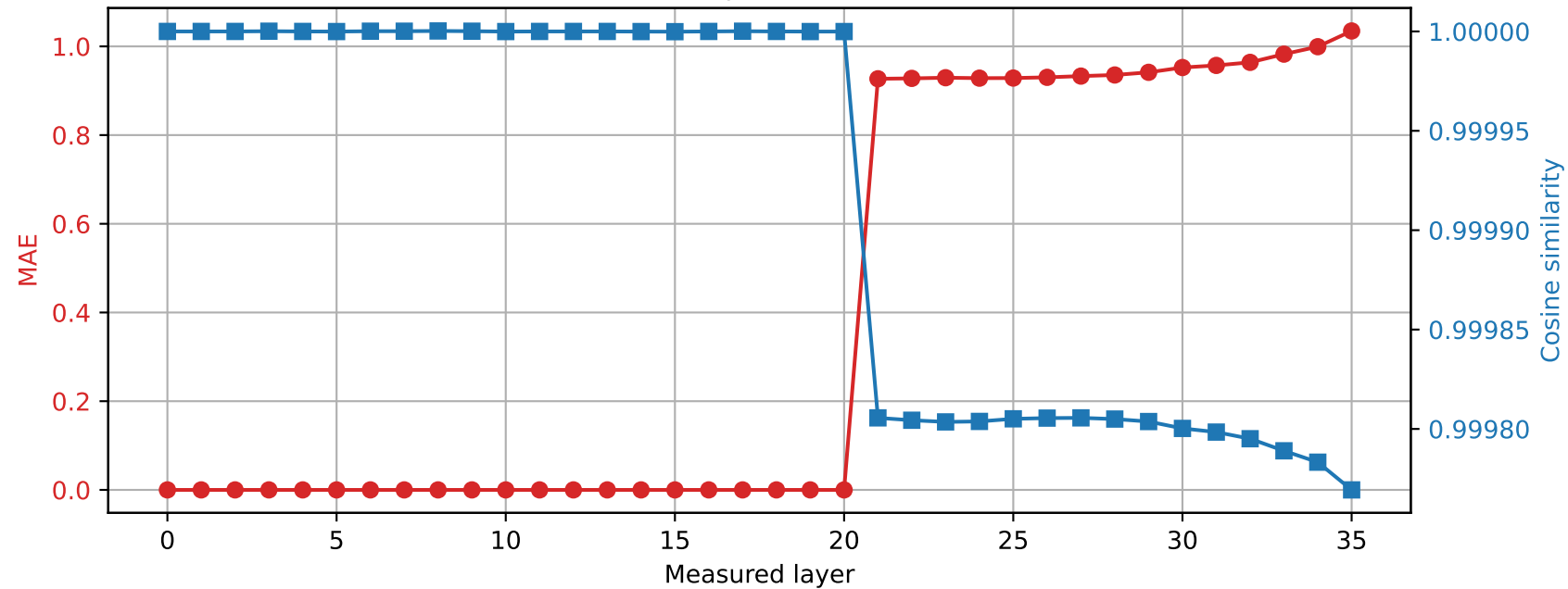
Qwen2.5-3B | Prompt 0 Spared layer 20 | Hybrid vs quantized
