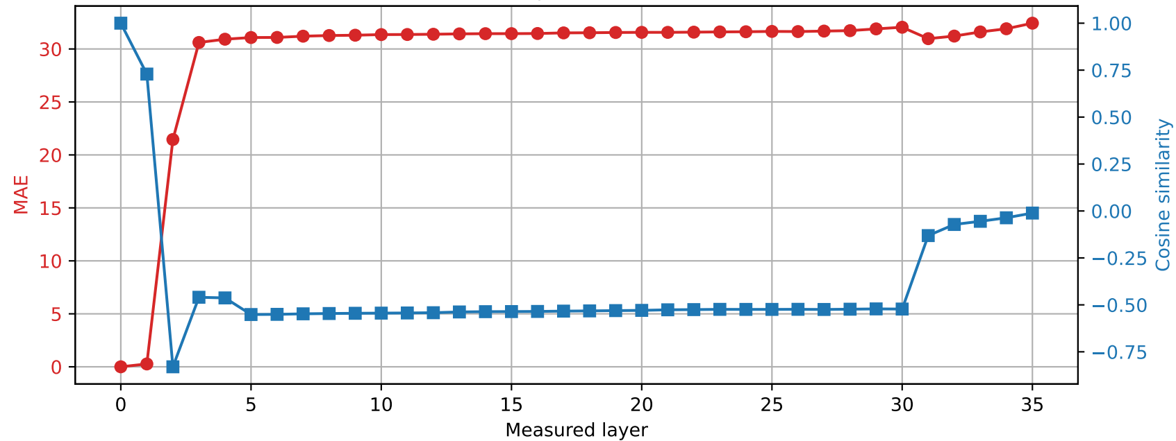
Qwen2.5-3B | Prompt 0 Spared layer 20 | Hybrid vs unquantized
